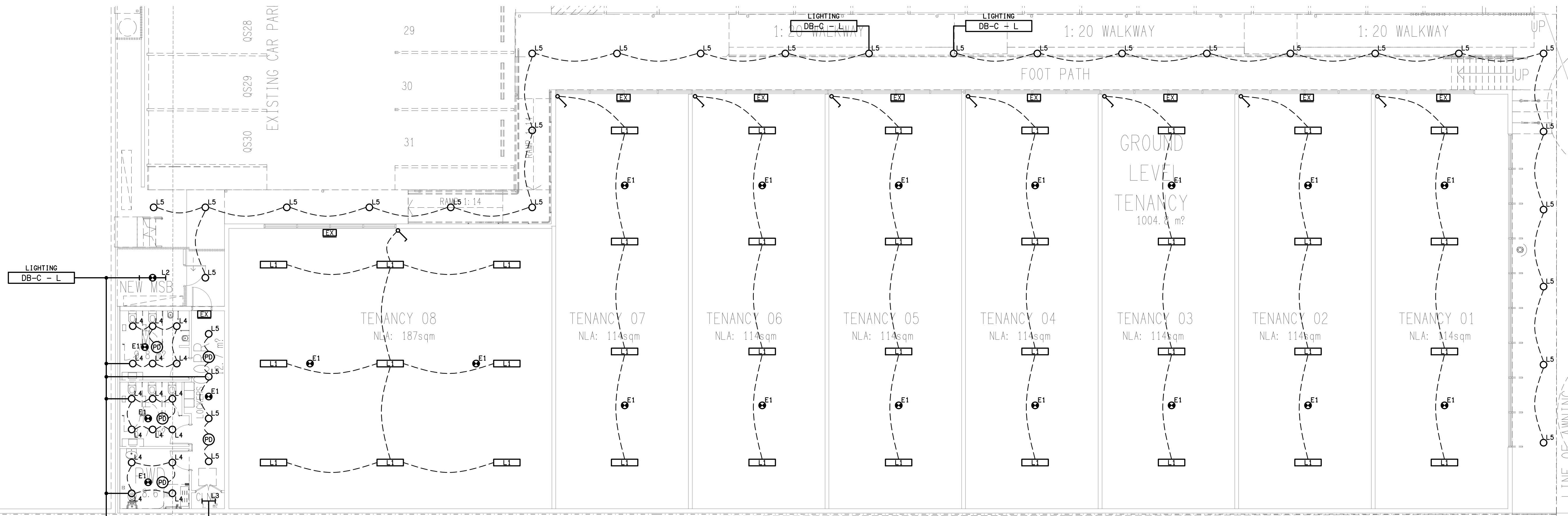
REFLECTED CEILING PLAN PROPOSED TENANCIES SCALE 1:100
