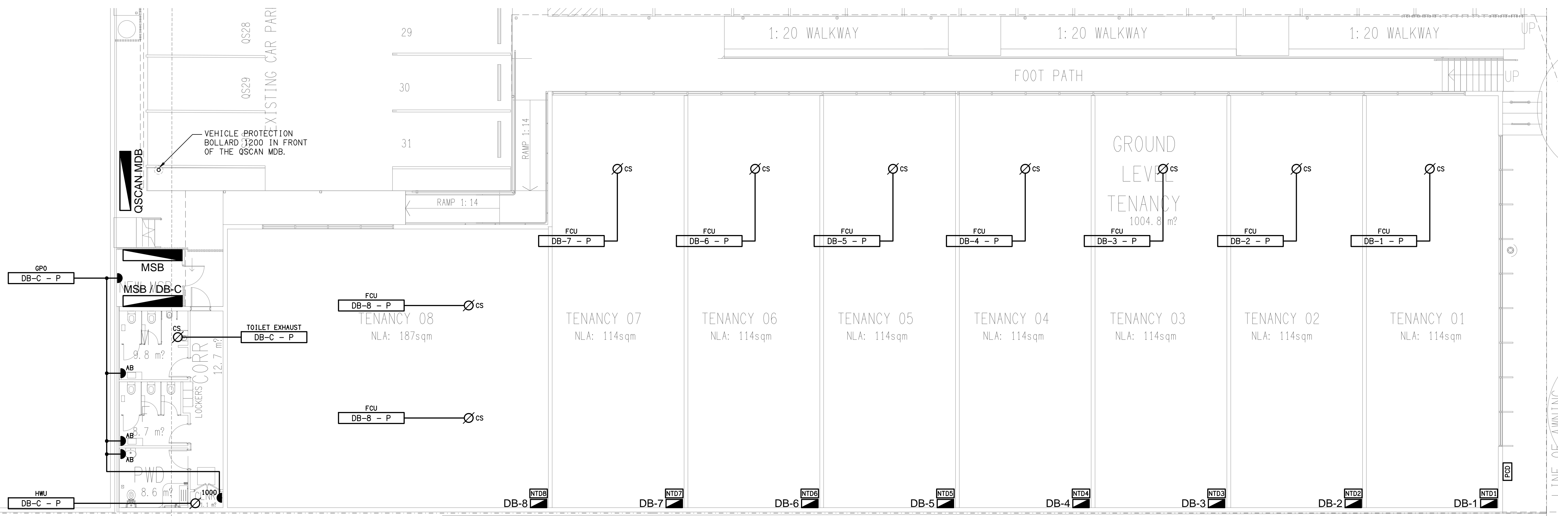
FLOOR PLAN PROPOSED TENANCIES SCALE 1:100
